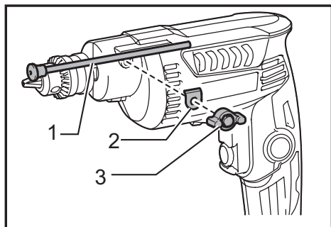
► 1. Depth gauge 2. Washer 3. Clamp screw
