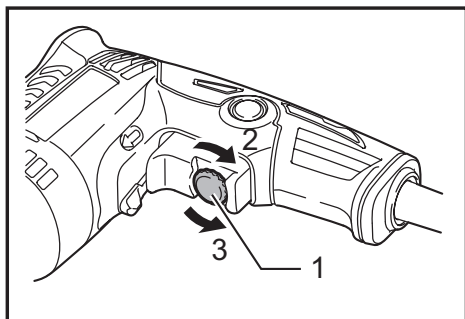
► 1. Speed control screw 2. Higher 3. Lower
